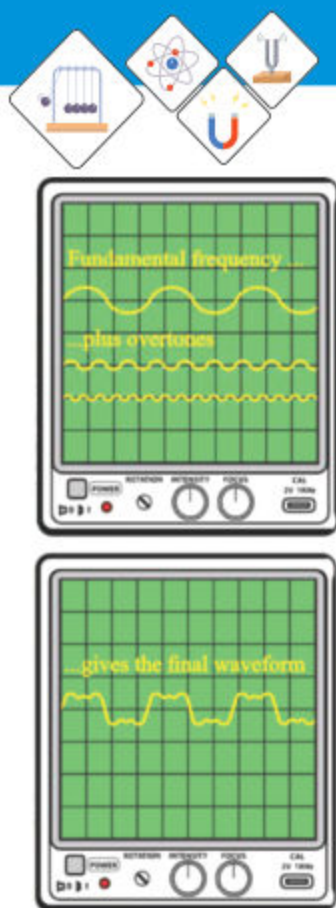
Fig: 11.6 Formation of a note on the oscilloscope
